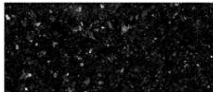
Star galaxy
